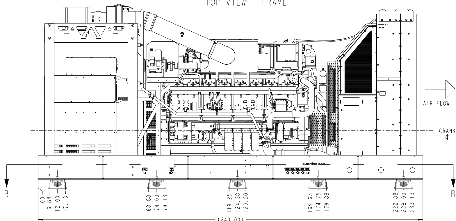
SECTION B-B TOP VIEW - FRAME
