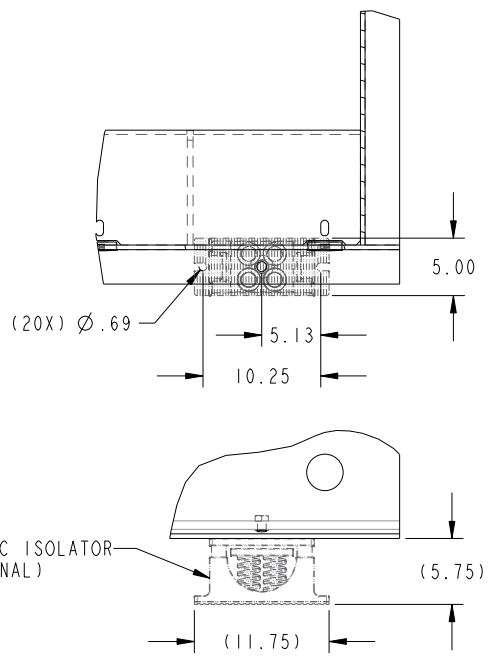
DETAIL D SCALE 1/125
